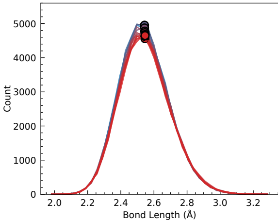
Cr-Ni Bond Length Distribution
